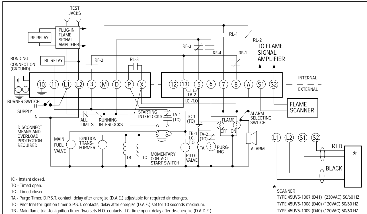
FIGURE 3. TYPICAL SCHEMATIC DIAGRAM FOR SEMI-AUTOMATIC PILOT IGNITED GAS OR OIL BURNER WITH PREPURGE, PILOT TFI, MAIN FLAME TFI AND INTERRUPTED PILOT
